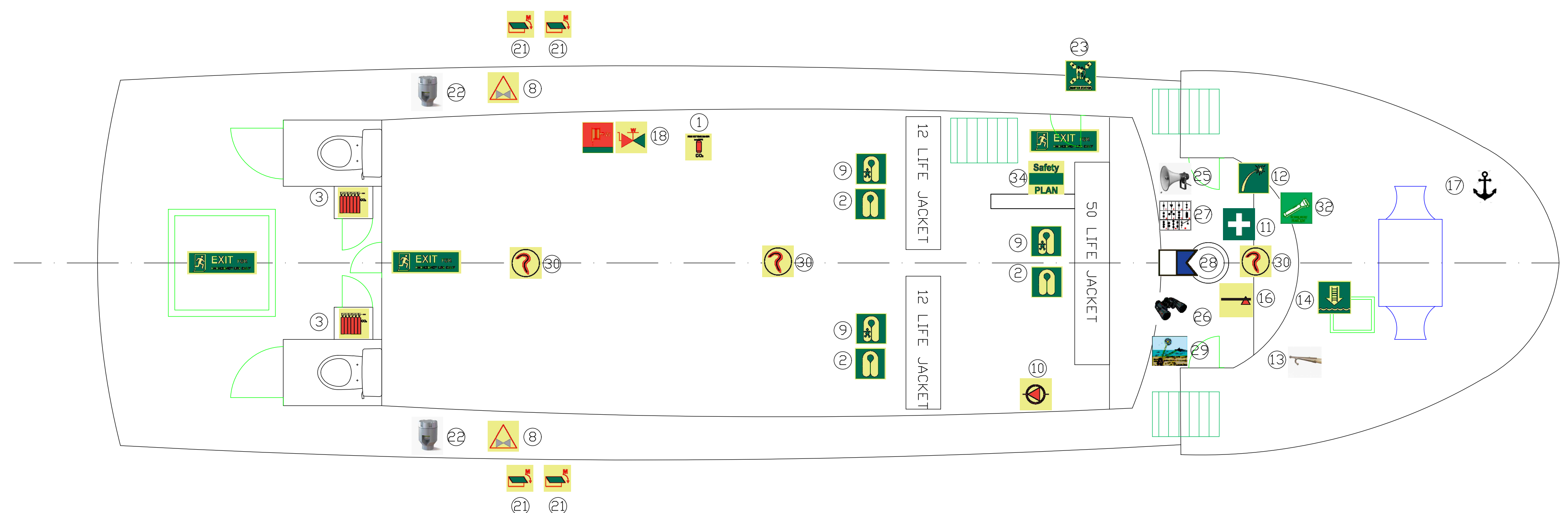
MAIN DECK
